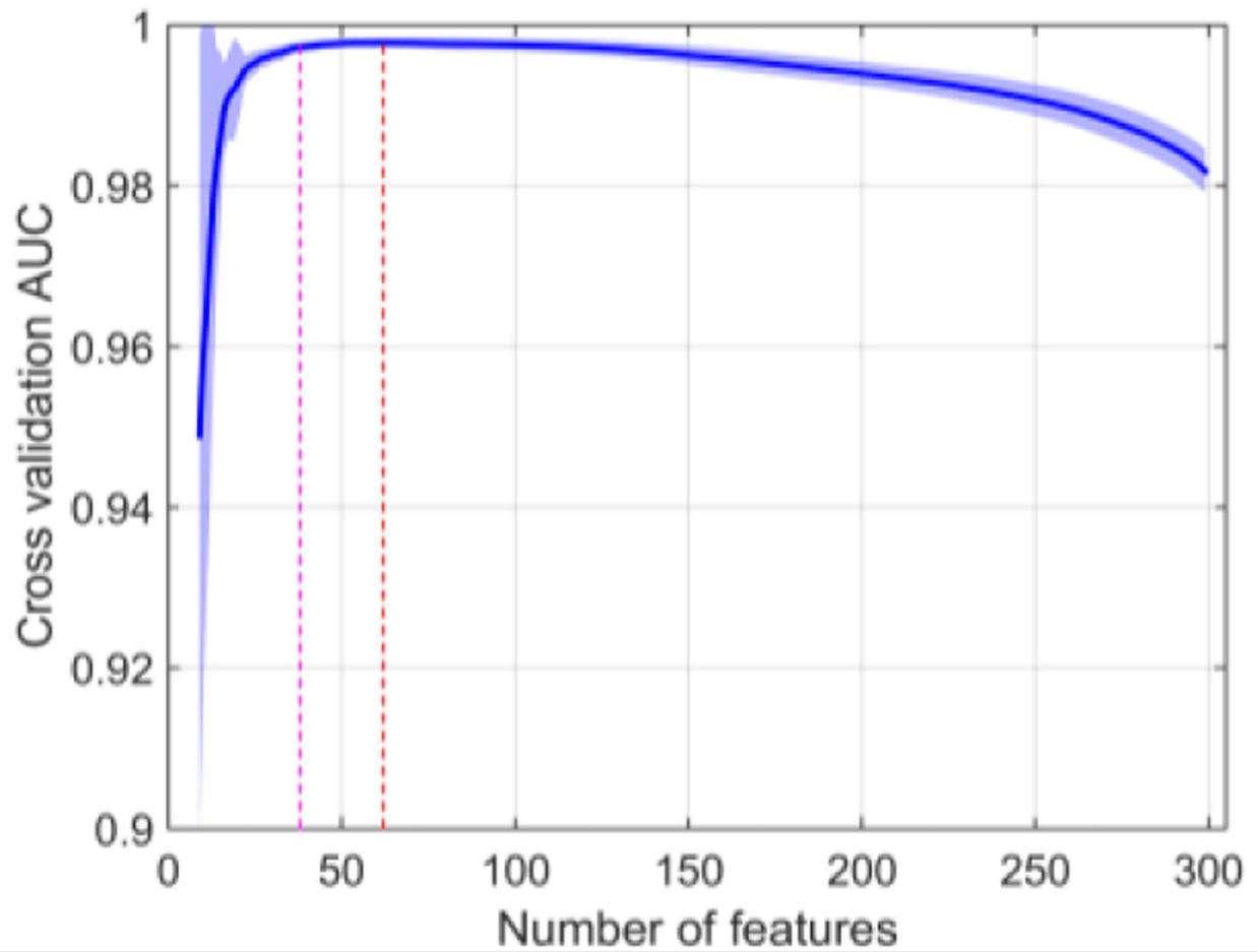
Fig. 2. Backward sequential feature selection performance curve calculated with respect to the testing data using 500 rounds of repeated random subset cross validation (CV). The average AUC value is shown as a solid blue line, and the 95% confidence intervals are shown as pale blue shading.
