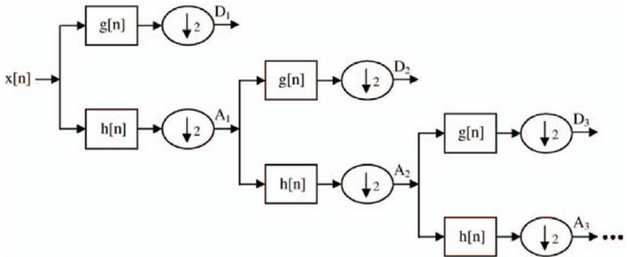
Fig. 3. Subband decomposition of discrete wavelet transform implementation [12].
