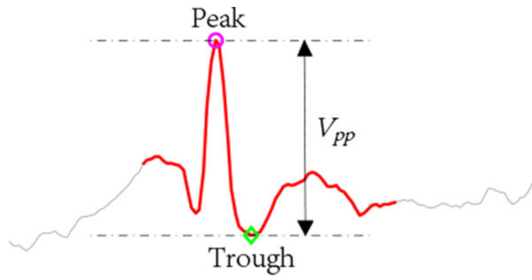
Figure 11. The peak-to-trough value V_{PP} of a spike.
