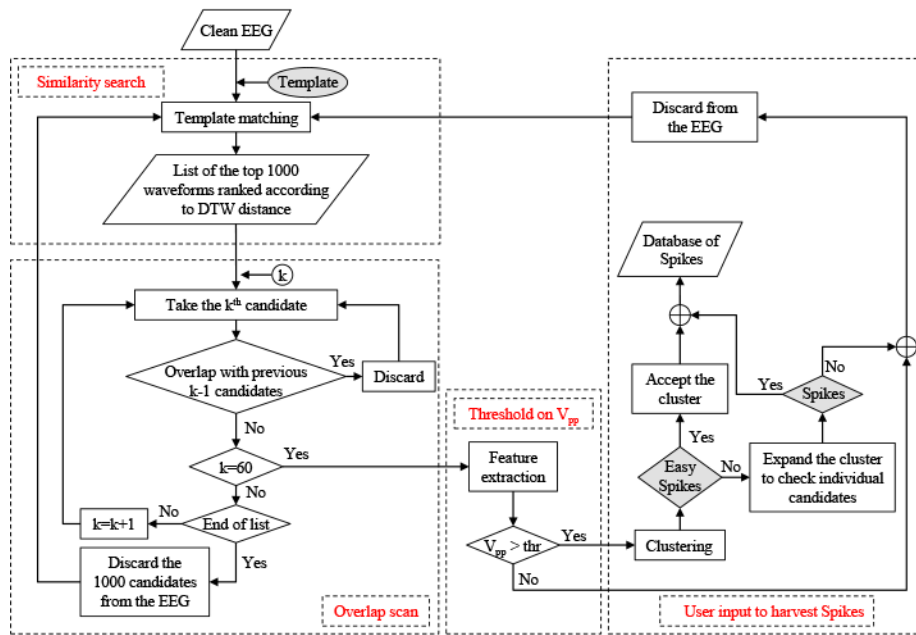
Figure 10. Flowchart of the proposed algorithm for rapid waveform annotation.
