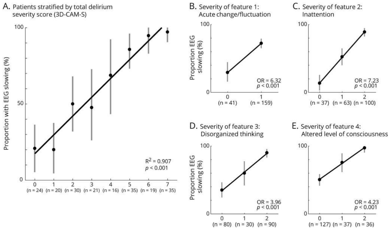
(A) Patients were stratified by 3-Minute Diagnostic Interview for Confusion Assessment Method delirium severity (3D-CAM-S) scores, and the prevalence of generalized EEG slowing was calculated at each score. Black line indicates fit by linear regression (adjusted R^2 = 0.907 , p < 0.001 ). Gray vertical lines indicate the bootstrap confidence intervals for each stratum (2.5%–97.5% percentiles of 1,000 bootstraps). (B–E) Patients were additionally stratified by the severity score of each individual 3D-CAM-S delirium feature (1–4), and the prevalence of generalized EEG slowing was calculated at each score. Logistic regression was used to quantify the relationship between delirium feature severity (dependent variable) and EEG slowing (independent variable). Severity of each delirium feature was significantly associated with EEG slowing (all odds ratio [OR] > 1, p < 0.05 ).
