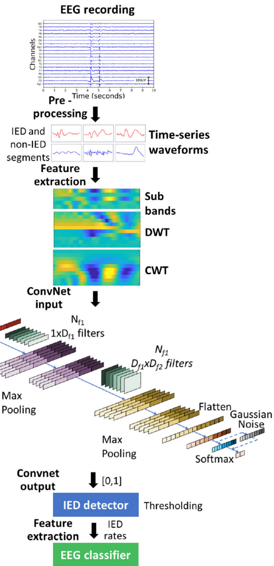
Fig. 2. Overall workflow of the ConvNet IED detector and EEG classifier. The proposed 1D ConvNet architecture has two convolutional, pooling and fully connected layers with multiple input features. During training, Gaussian noise is added to the last fully connected layer, before the softmax function.
