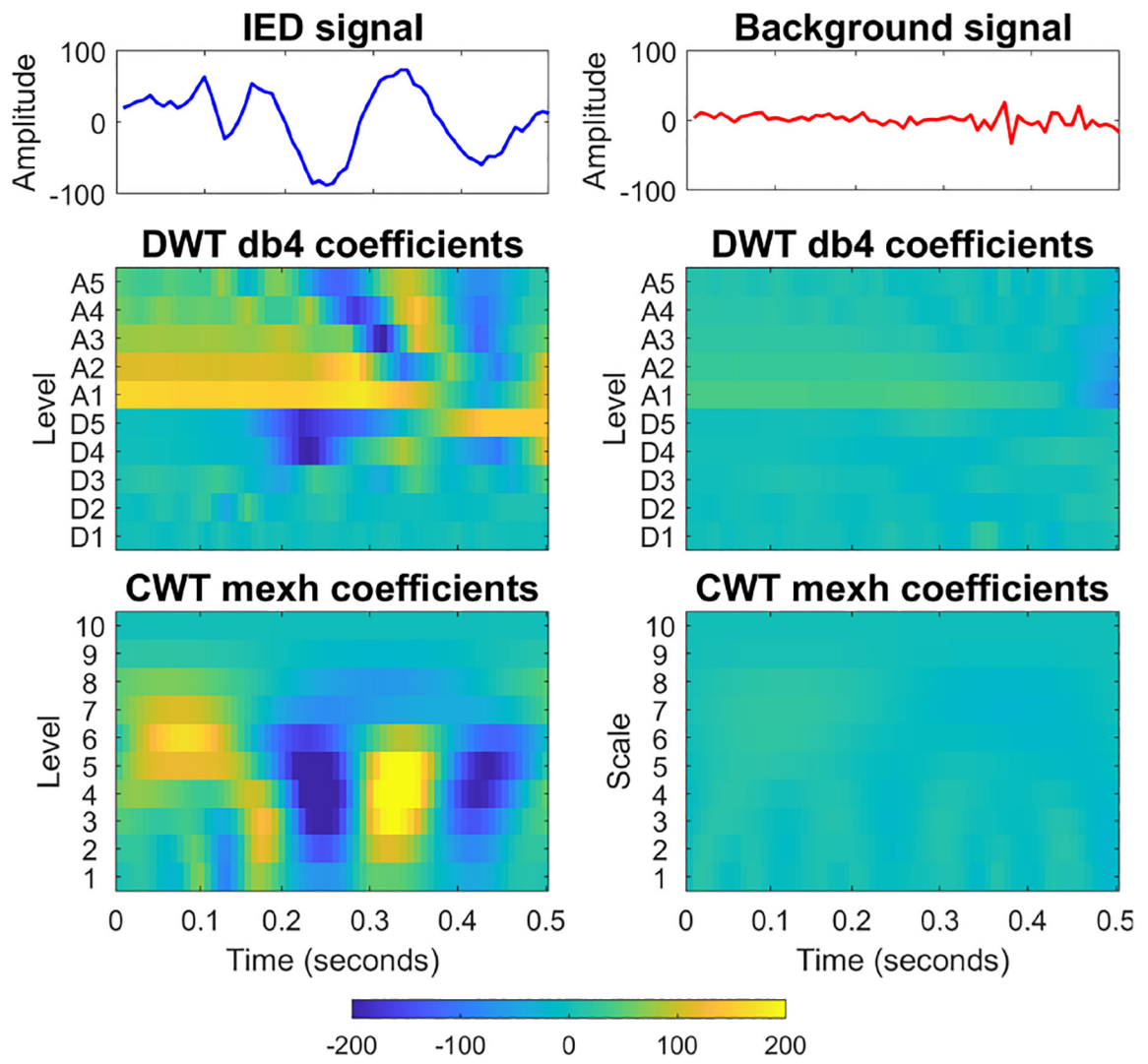
Fig. 1. db4 and Mexican hat wavelet coefficients (magnitude) for IED and background segments.
